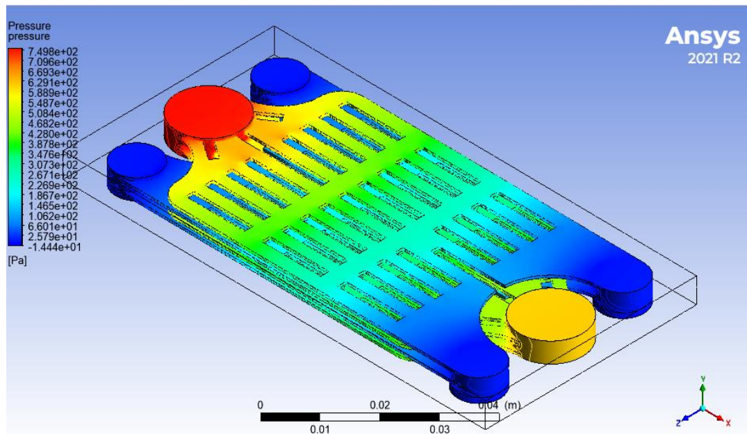
Figure 14: Pressure contour
