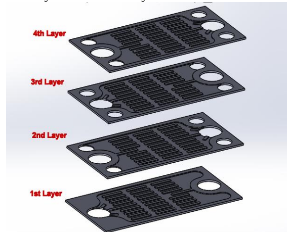
Figure 1: Exploded view in Solidworks of Microchannel heat Exchanger
