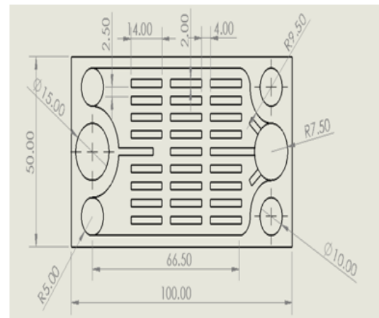
Figure 2: Dimension of single plate in mm
