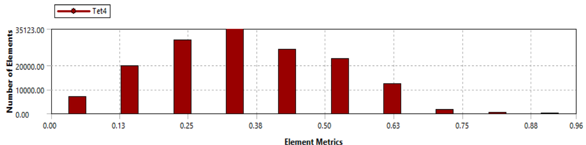
Figure 6: Skewness Graph
