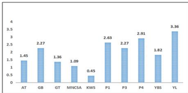
Fig.4: Chemical Oxygen Demand (COD) of various water samples
