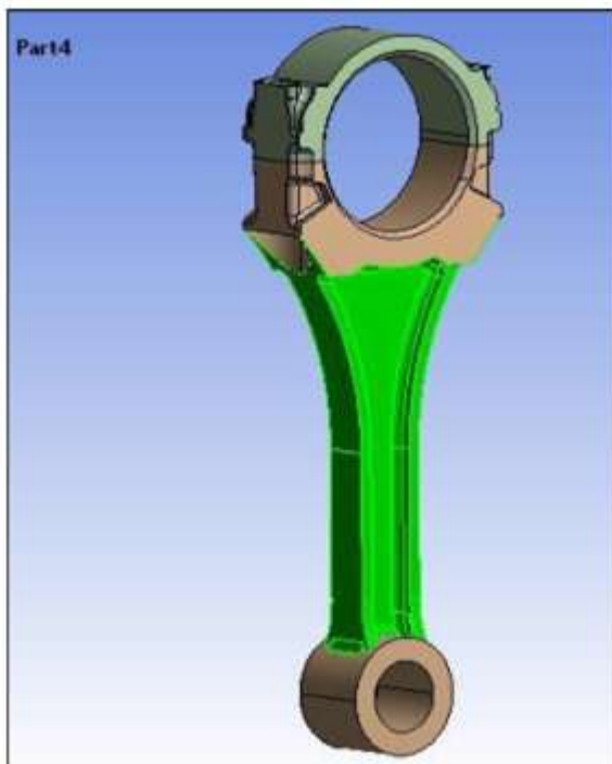
Fig. 15. Reinforcement on I section
