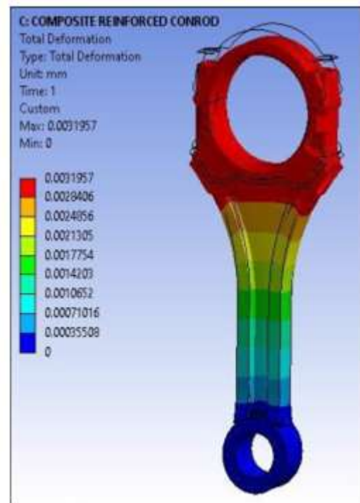
Fig. 16. Total deformation Result
