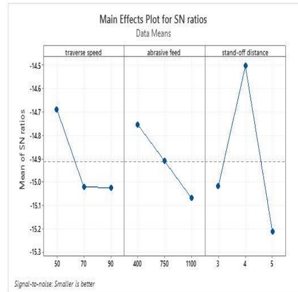
Figure 4. Taguchi results for lower SR
