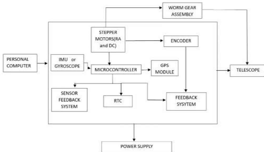
Fig. 2. Block Diagram
