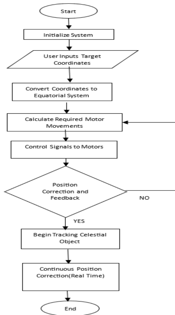
Fig. 1. System flowchart
