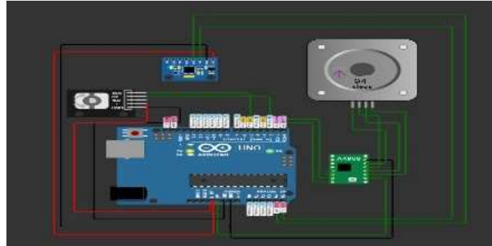
Fig. 5. Simulated circuit
