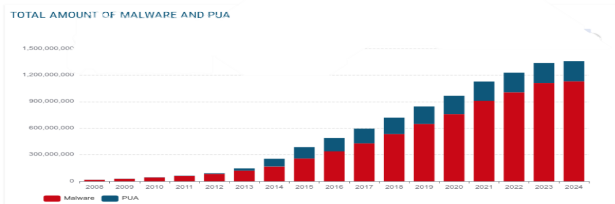
Fig.4.Total Malware
