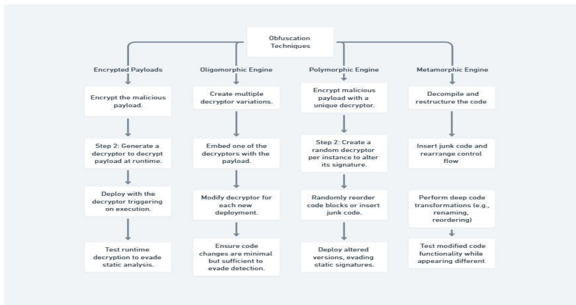
Fig.2.Obfuscation Techniques
