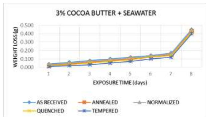
Figure 16: Graph of 3% Cocoa Butter plus Seawater
