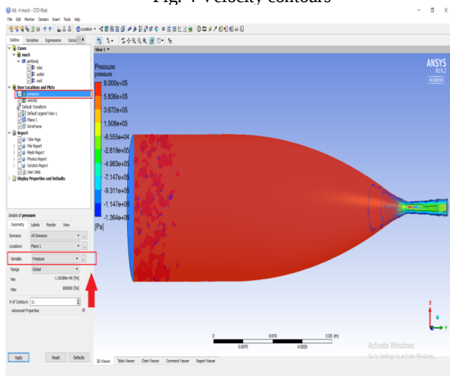
Fig. 5 Pressure contours
