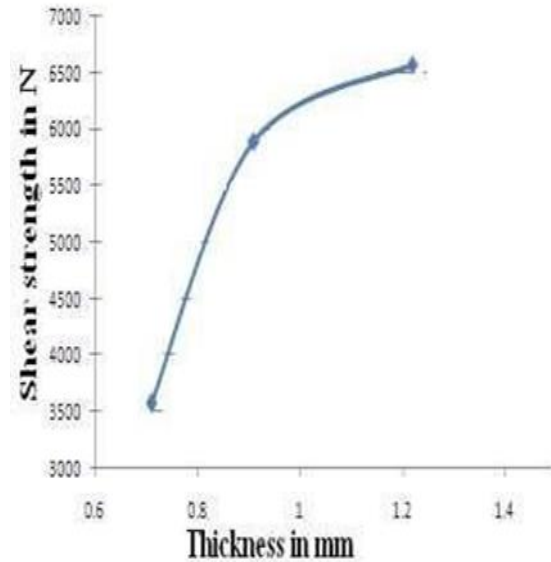
Fig 8 Relationship between specimen thickness and shear strength
