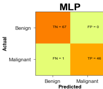
Fig. 7. Confusion Matrix of MLP
