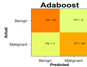
Fig. 9. Confusion Matrix of Adaboost
