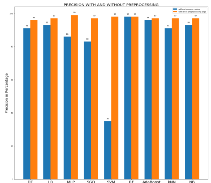
Fig. 17. Precision with and without preprocessing
