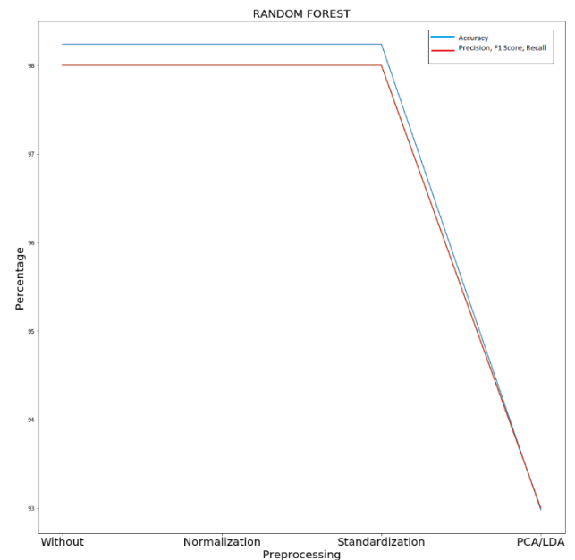
Fig. 20. Preprocessing graph for random forest
