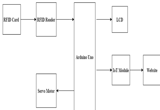
Fig. 1. Block Diagram showing hardware modules connected to Arduino Uno
