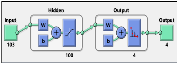
Figure 1: Model Recognition Artificial Neural Network Architecture
