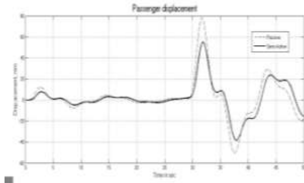
Fig 9: Passenger displacement for double bump.
