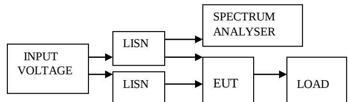
Fig 1. Block diagram for emission testing
