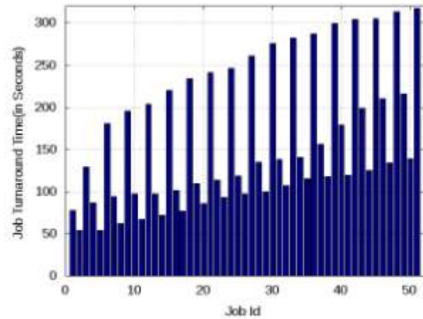
Figure 3: Jobs and turnaround time (in seconds) using Non Rule Based Approach.
