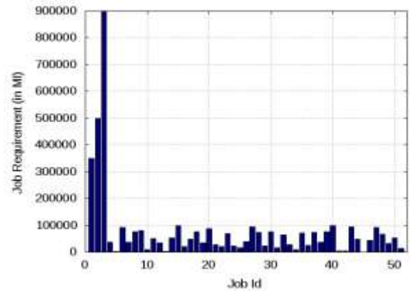
Figure 2: Jobs and requirement (in Million Instructions).
