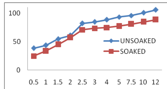
GRAPH. 3.9 CBR TEST FOR 3% OF AGAVE SISALANA FIBER
