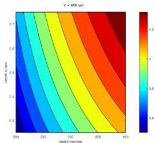
Figure 2: Roughness for different depth and feeding at speed 600 rpm
