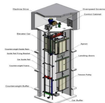
Fig. 1. Construction of elevator
