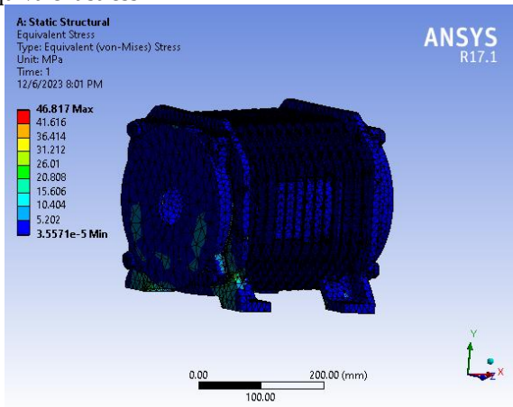
Fig. 5. Equivalent stress
