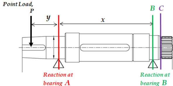
Fig. 4. Load Calculation
