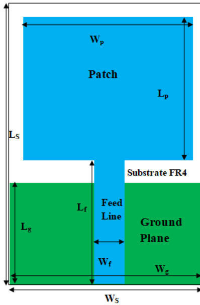
Fig. 1: The geometrical structure of the reference microstrip UWB antenna
