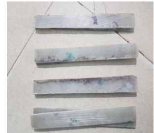
Fig 13: Glass epoxy laminate specimen of varying orientations
