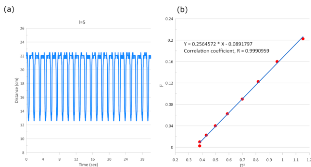
Fig 3. (a) Distance vs time response measured for the case of length of 5cm of suspension from the pendulum. The peak to peak time for an entire cycle is measured from the curve. b) l^2 vs l/T^2 plot with fitted equation of a line to extract the slope and intercept. Acceleration due to gravity is extracted using the slope and Radius of gyration is extrapolated using intercept.
