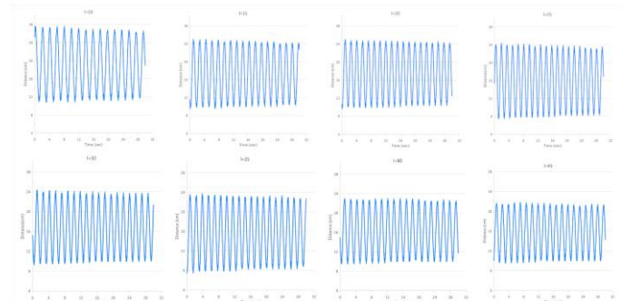
Fig. 4. Simple harmonic data from Board Echo measurement for various lengths l of the bar pendulum
