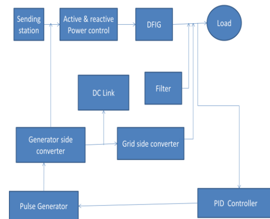
Fig 1 Block Diagram of offshore wind turbine system
