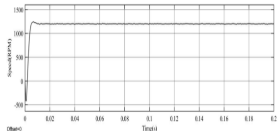
Figure 12.c: Speed 1200rpm
