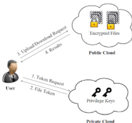
Fig. 3. De-duplication approach in cloud storage network[13]
