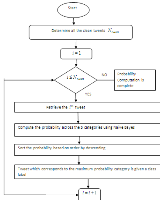
Fig. 7. Probability Computation
