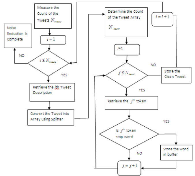
Fig. 6. Noise Reduction Process
