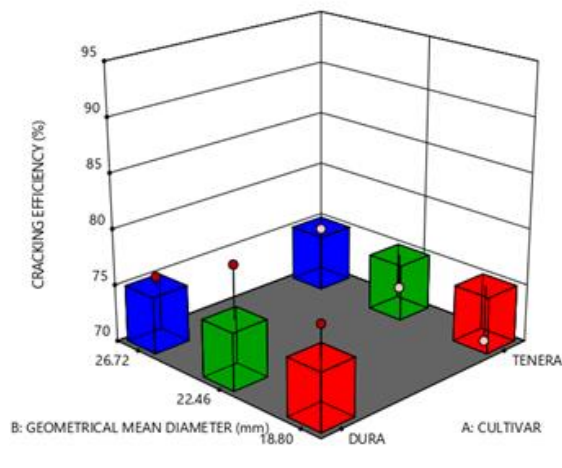
Figure 10: Optimum cracking efficiency at drying temperature of 15 hrs for both cultivars.
