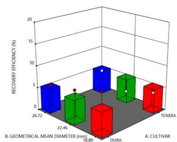
Figure 19: Optimum recovery efficiency at drying period of 18 hrs for both cultivars.
