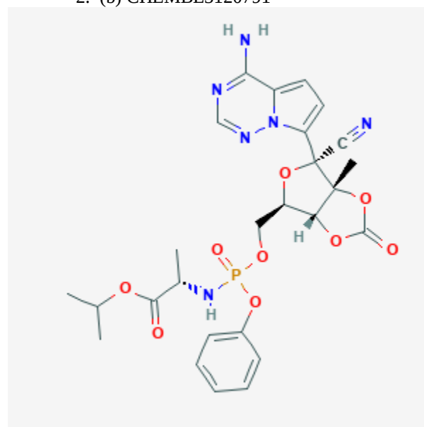
Fig 3. Structural differences with Uprofosbuvir, SCHEMBL20762917 and SCHEMBL20733228.
