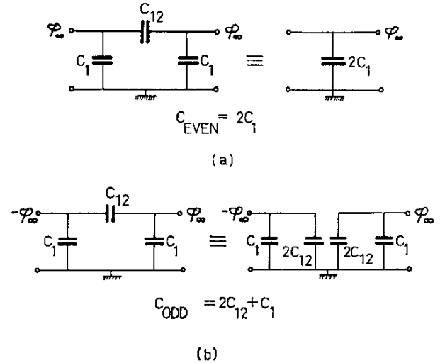
Figure 2. (a) The even mode equivalent circuit for the gap capacitance.
