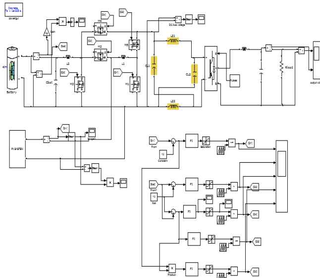
Fig.5. Simulation diagram of proposed system
