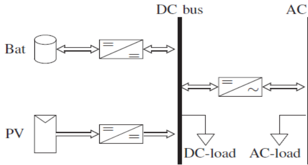
Fig.2. Three port Dc-Dc converter
