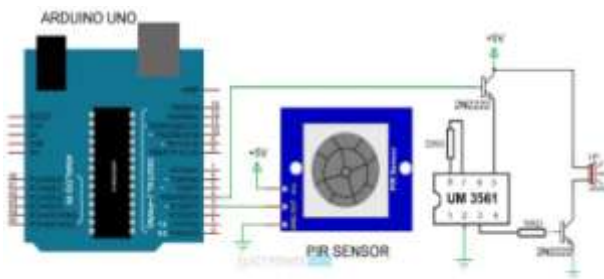
Fig 2: Proposed Architecture
