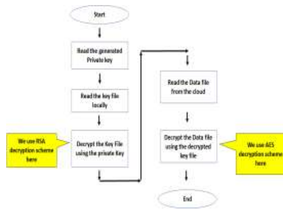
Figure.3: File Read Operation
