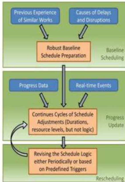
Fig. 3 Predictive-reactive scheduling
