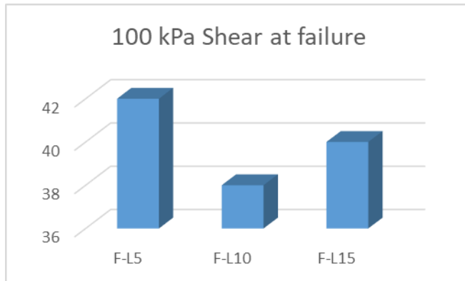
Fig. 3 Shear failure under 100 kPa normal stress.
