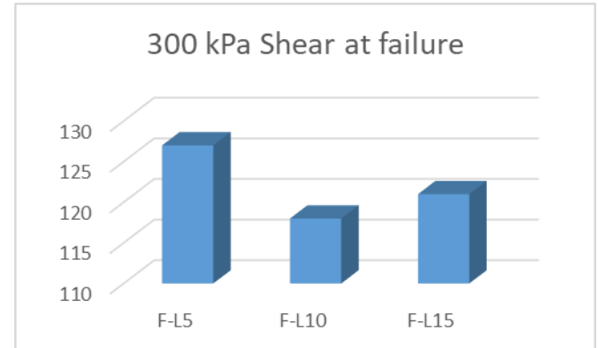
Fig. 5 Shear failure under 300 kPa normal stress.
