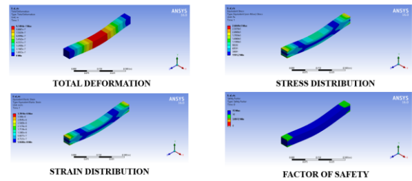
Fig 6. Result of Aluminium Alloy
