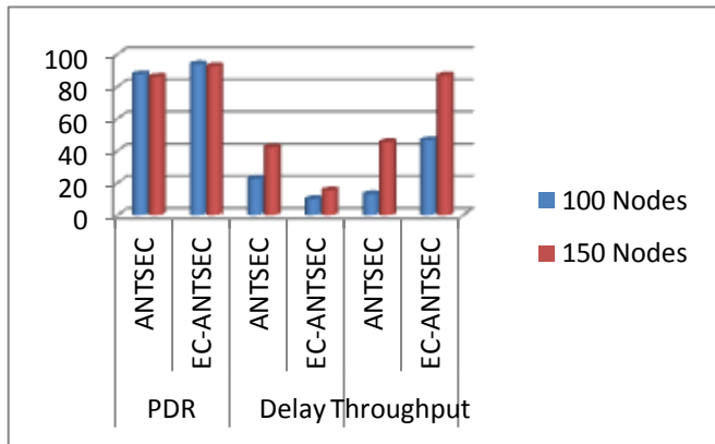
Fig 5: Comparison of ANTSEC AND EC-ANTSEC Framework with 100 and 150 nodes
