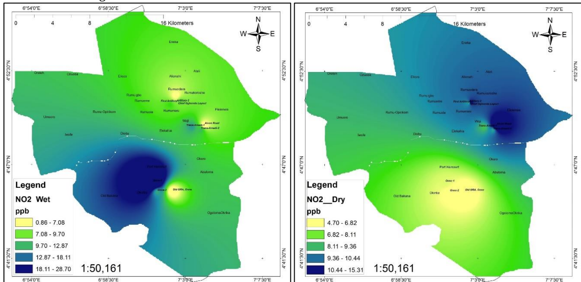
Figure 5: Spatiotemporal Variation of NO 2 (ppb)
