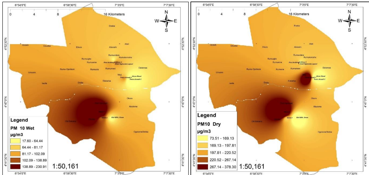
Figure 3: Spatiotemporal Variation of PM 10 (µg/m 3 )
