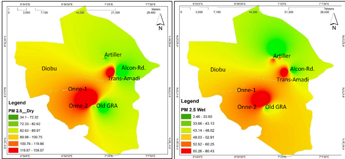
Figure 4: Spatiotemporal Variation of PM 2.5 (µg/m 3 )
