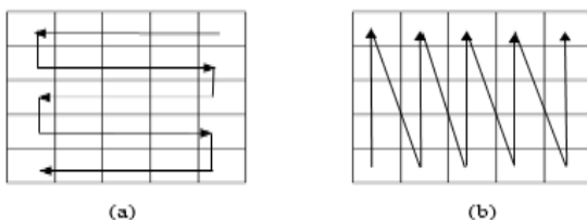
Fig. 1. Scan pattern 1 (a) encryption (b) encoding
