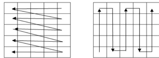
Fig. 2. Scan pattern 2 (a) encryption (b) encoding
