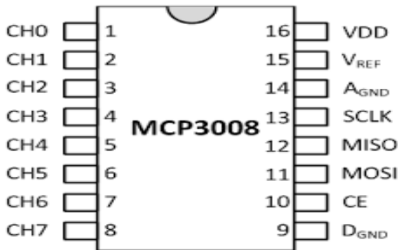
Fig.3. Pin Configuration of ADC (Mcp3008)
