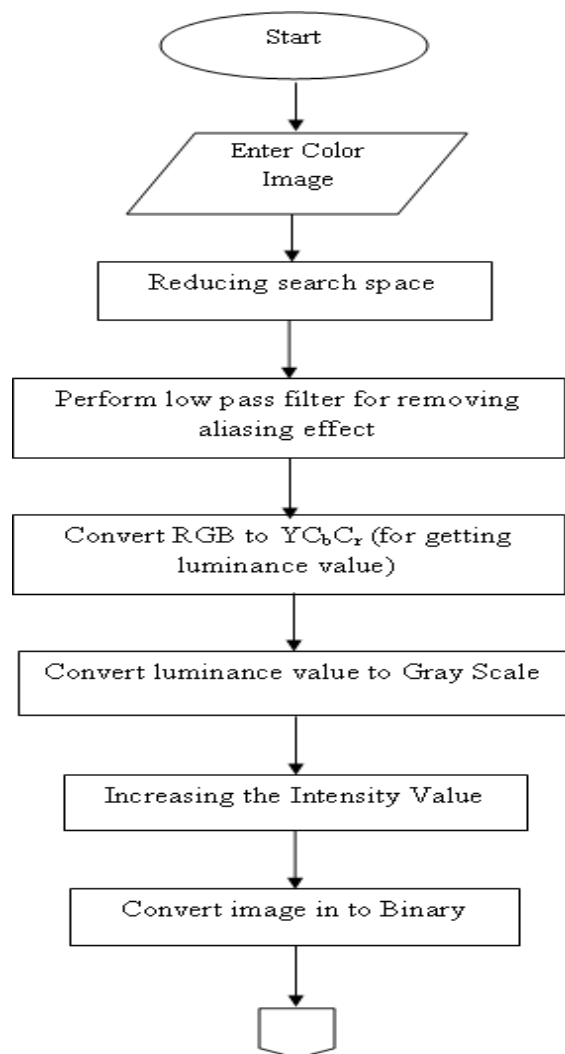
Figure 1.2: Algorithm for Extracting facial features from Occluded region Images.
