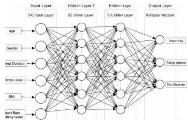
Fig. 1. FNN Architecture
