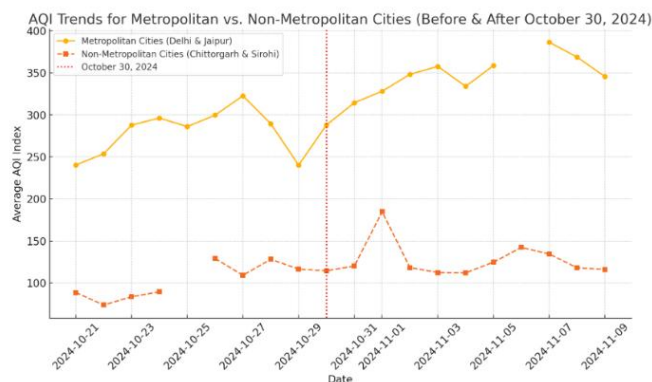
Fig.3. AQI trends Metropolitan Cities and Non-Metropolitan Cities (before and after October 30, 2024)
