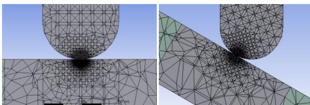
Fig. 5: Cross-sectional view of the mesh for the normal and oblique impact of the rod
