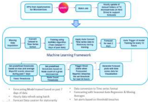
Fig. 1. Novel AIOps Framework
