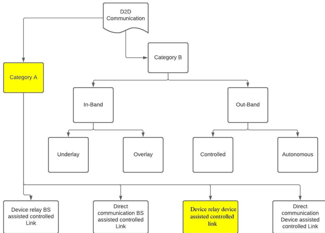
Figure1.1 D2D Classification
