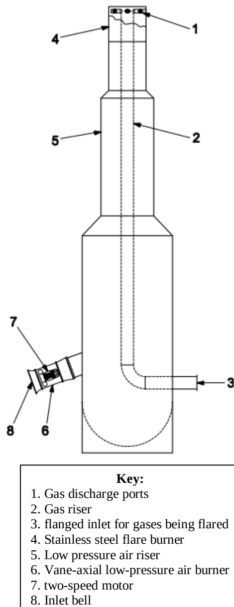
Fig.2. Air-assisted Flare [7]
