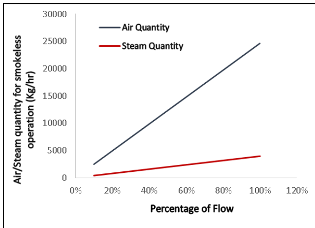
Fig. 3. Air/Steam quantity required for different percentage of flow for Butane (C 4 H 10 ) for smokeless operation.
