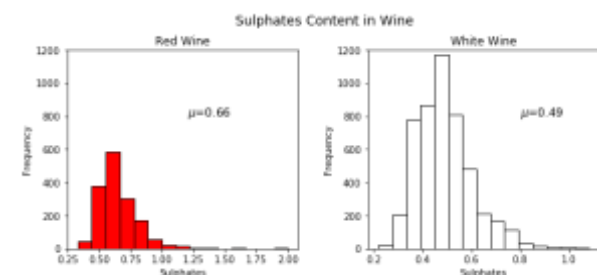
Fig 9: Sulphates content
