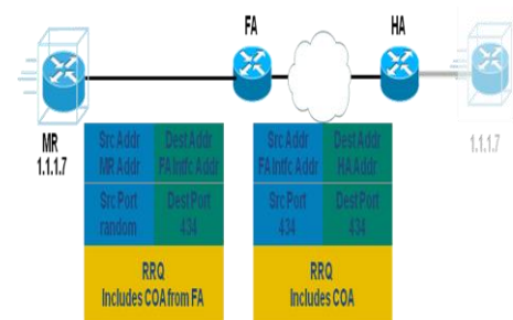
Fig.4. Sending RRQ
