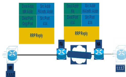
Fig.5. RRQ Reply
