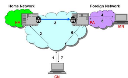
Fig.1. Mobile IP Operation
