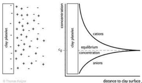
Fig. 2 Distribution of cations and anions adjacent to a clay platelet according to the diffuse double layer theory (Keijzer, 2000).
