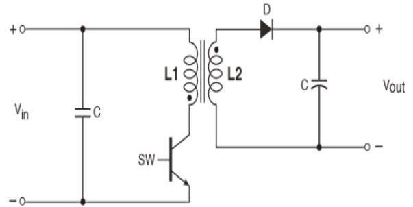
Fig 11- Flyback converter
