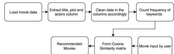
Fig 3. Workflow of the application
